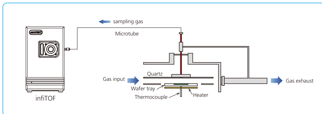
Fig. 1 Experimental setup of MOVPE reactor coupled to the infiTOF.
