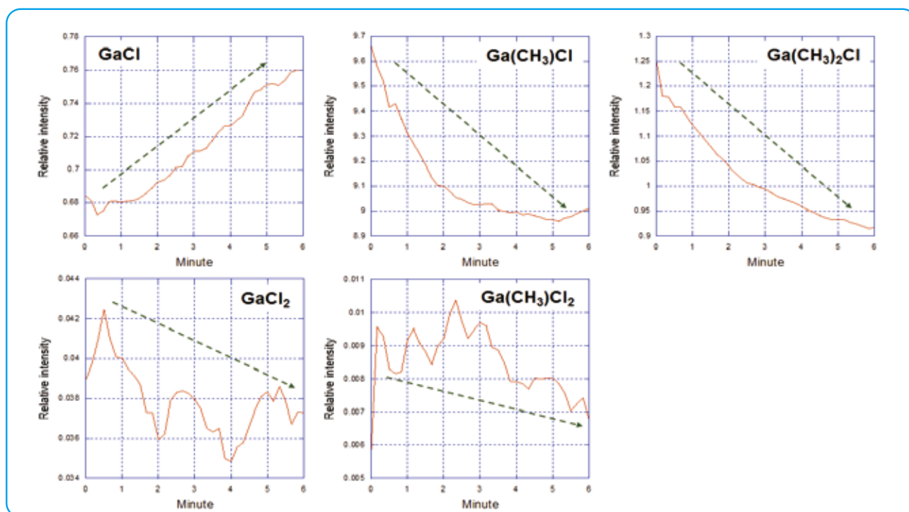
Fig.4 Normalized mass chromatograms of chlorine adducts.
