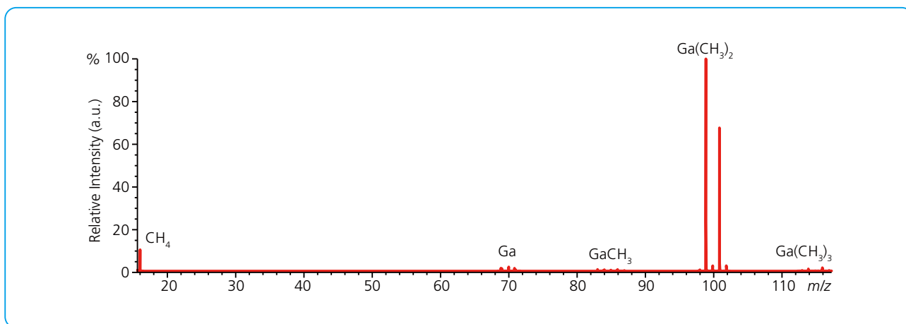
Fig. 2 Mass spectrum of TMG.
